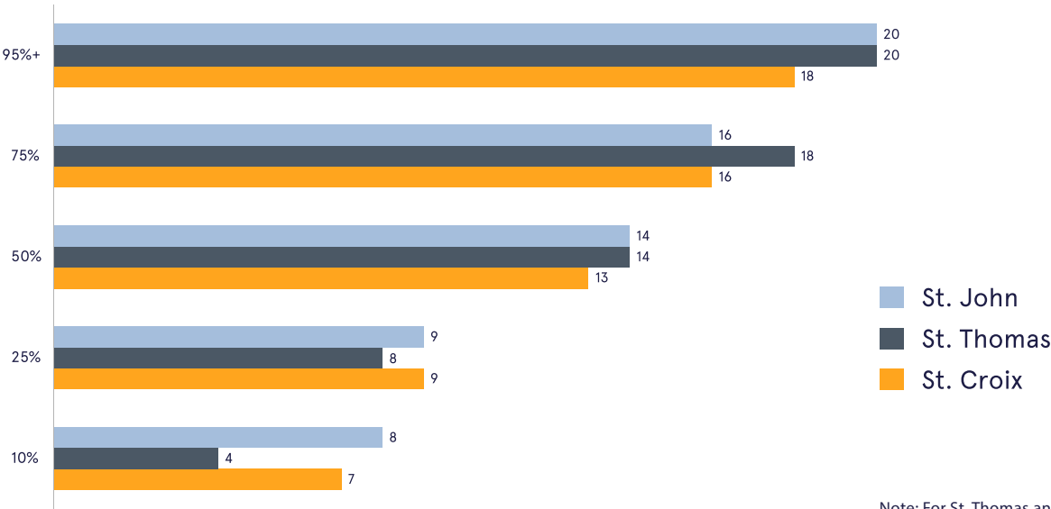
Time post-storm to reach a given level of WAPA customer restoration, by island % of eligible customers; number of weeks
