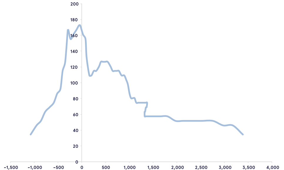
Wind speed at Hurricane Maria center (mph, vertical axis) vs. distance to downtown Christiansted (miles, horizontal axis) Source: Task Force analysis based on NHC data.
